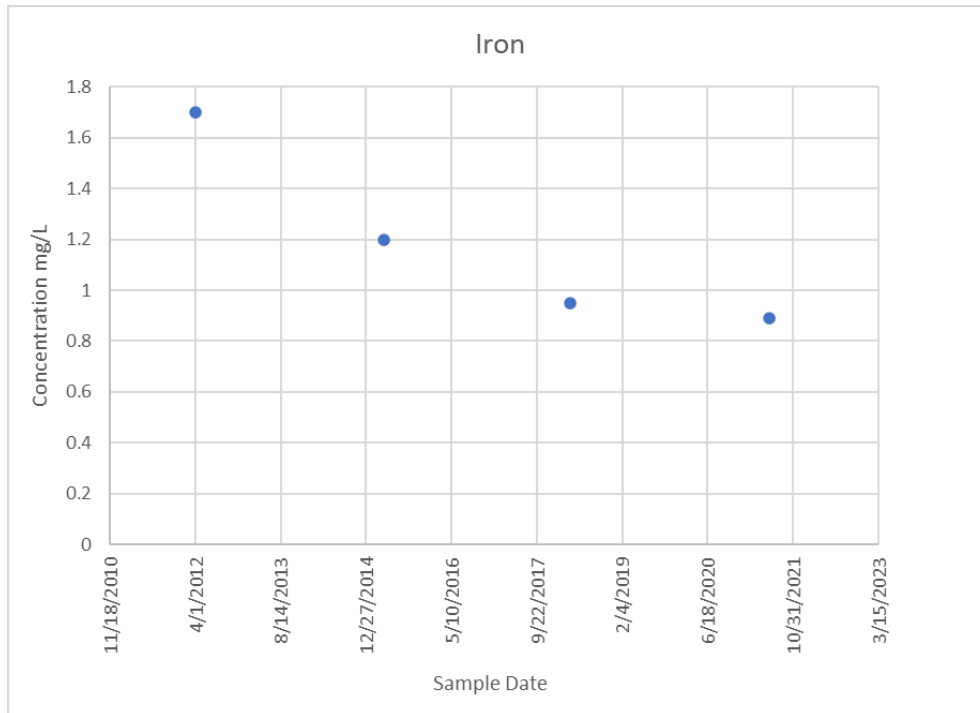
Exhibit 3-2: Iron and Sulfate Concentration Trends
